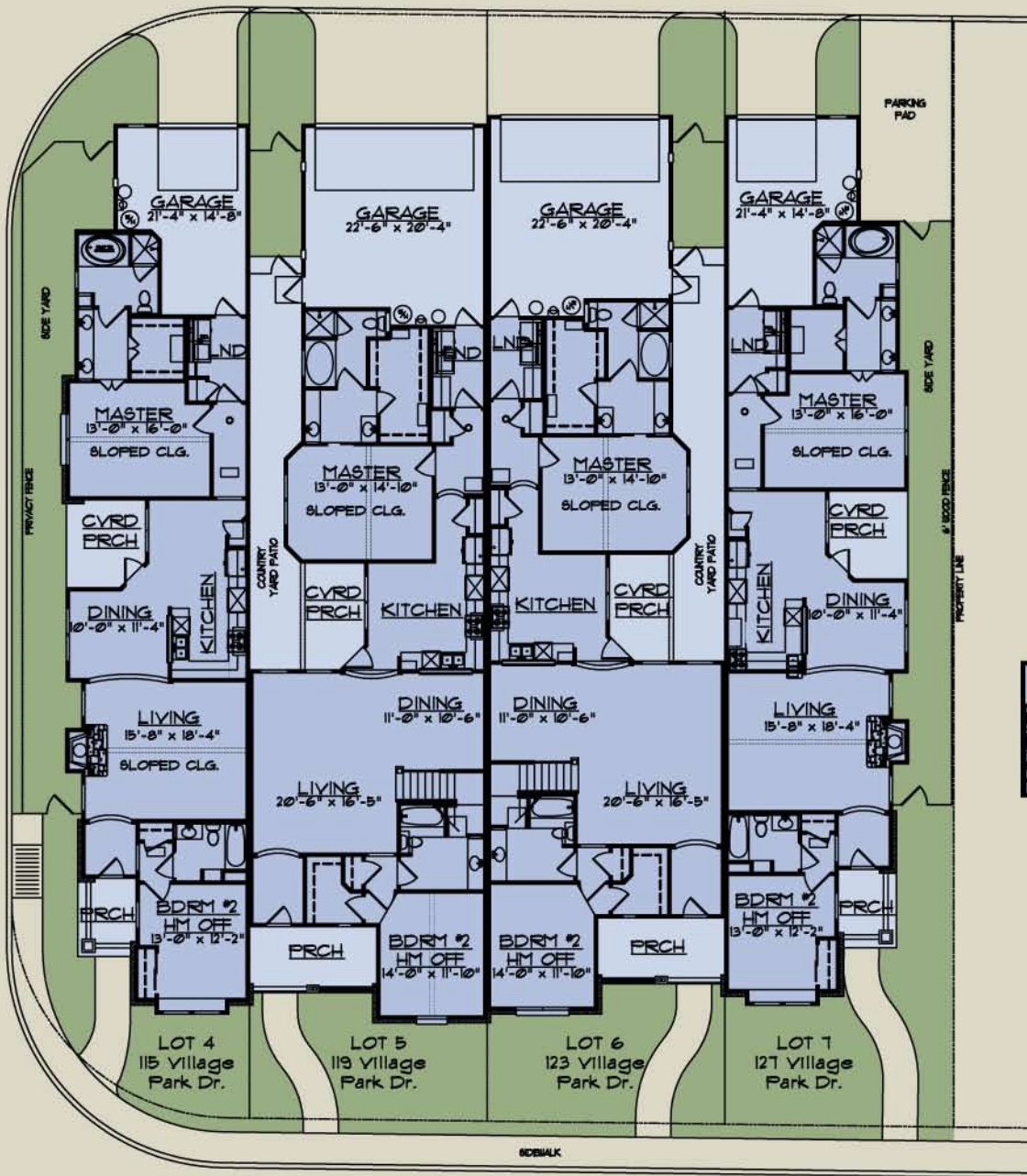
PLAN 1512 SQ. FT.
